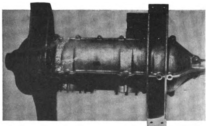
This Case Was Nearly Severed, But Welding Saved It.
